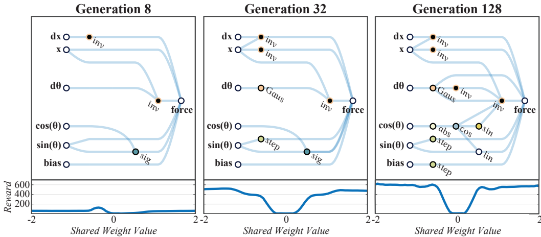
Figure 4: Development of Weight Agnostic Neural Network Topologies Over Time
